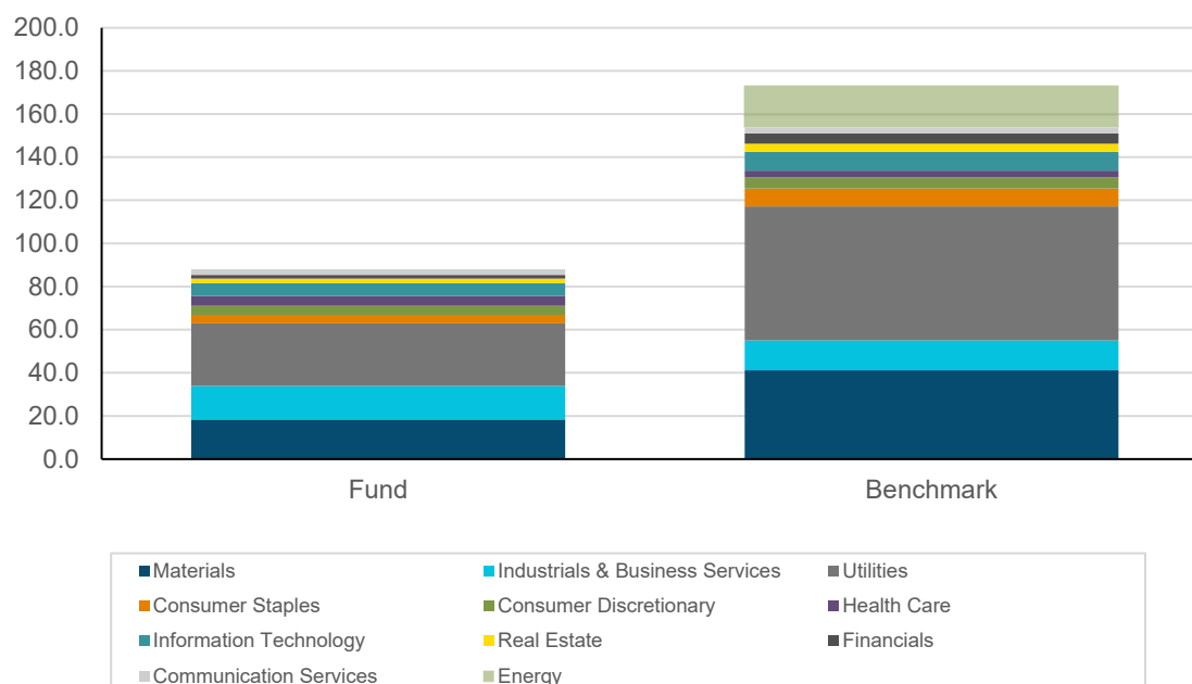
Weighted Average Carbon Intensity Contributions by Sector (mtCO 2 e / US$1 mn Revenue)
